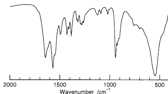
Figure 1. Infrared spectrum of [Mo 4 O 12 (glycylglycylglycine) 2 ]·9H 2 O.
